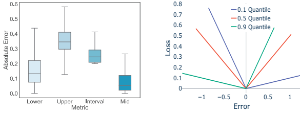
Figure 8: Box plot of related Figure 9: Quantile loss at 10^{th} , 50^{th} and 90^{th} quantiles.
